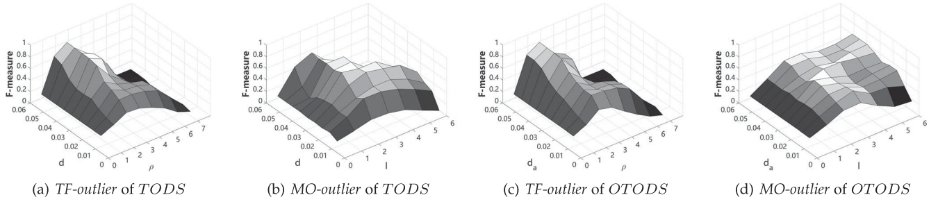
Fig. 12. F-measure (TaxiShanghai13).
