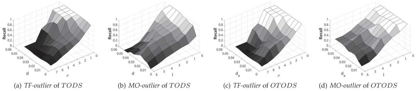
Fig. 11. Recall (TaxiShanghai13).
