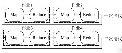
Fig.2 Job division of PageRank in two iterations
