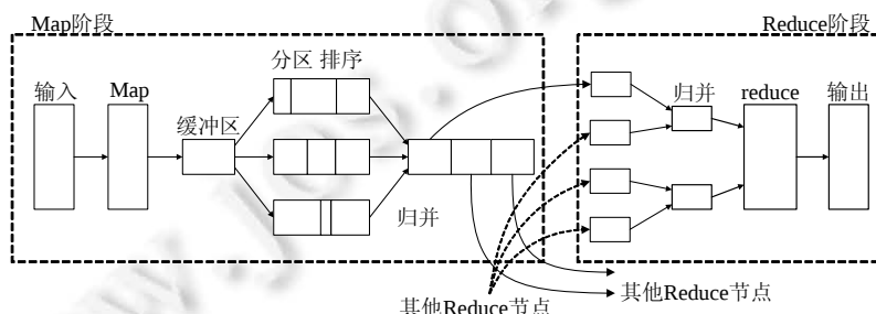
Fig.5 Implementation process of MapReduce
